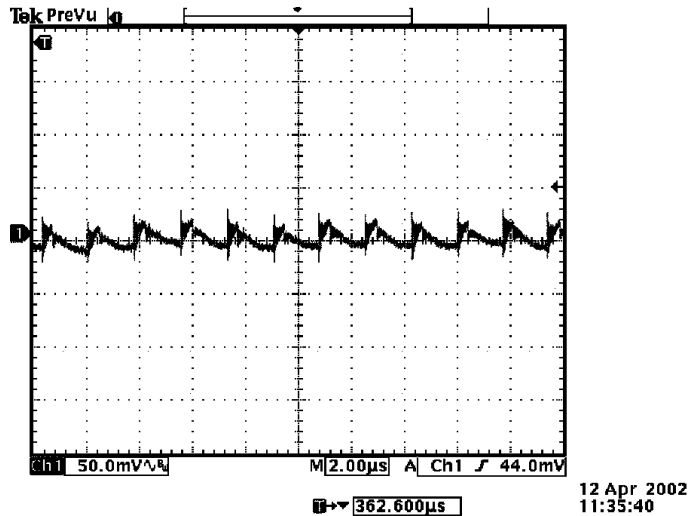
Ripple and noise at full load and 12.0Vdc input, and Ta=25° C with 560 µF external cap
