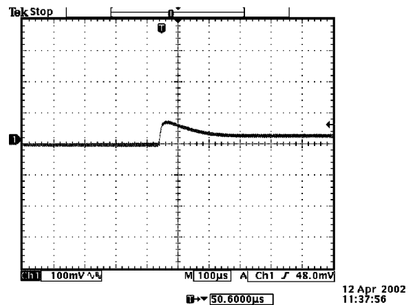
Vout=1.2V 100% to 50% load transients at 12.0V input and Ta=25° C
