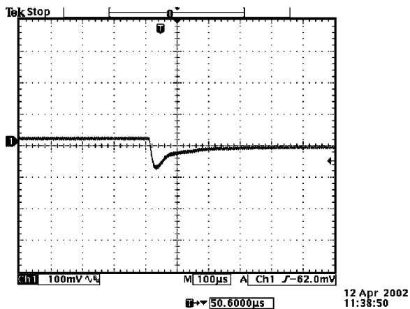
Vout=1.2V 50% to 100% load transients at 12.0V input and Ta=25° C
