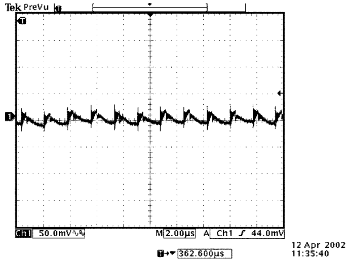
Ripple and noise at full load and 12.0Vdc input, and Ta=25° C
