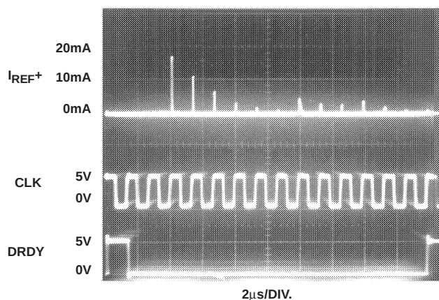
FIGURE 15. TYPICAL REFERENCE INPUT CURRENT
