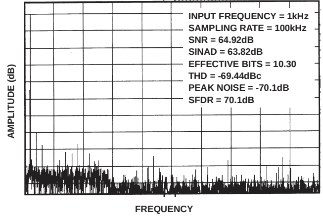
FIGURE 11. FFT SPECTRUM
