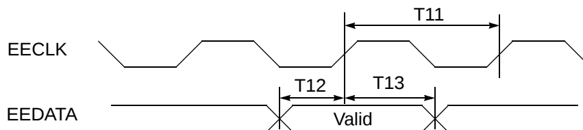
FIGURE 4. EEPROM timing
