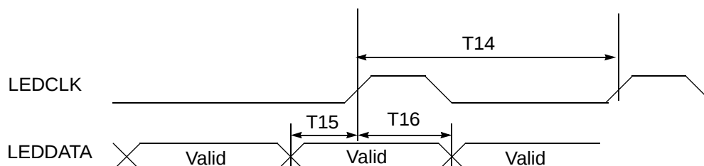
FIGURE 5. LED Interface
