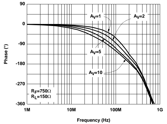
Non-Inverting Frequency Response (Phase) SO8 Package
