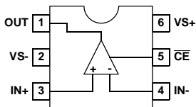
EL5193A (6-PIN SOT-23) TOP VIEW
