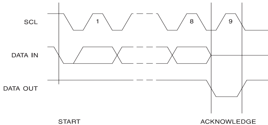
Figure 6. Output Acknowledge
