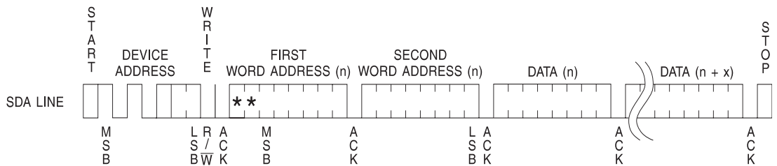
Figure 9. Page Write
