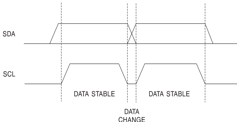
Figure 2. Data Validity
