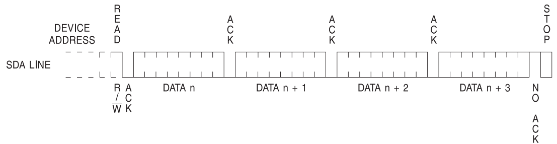
Figure 12. Sequential Read
