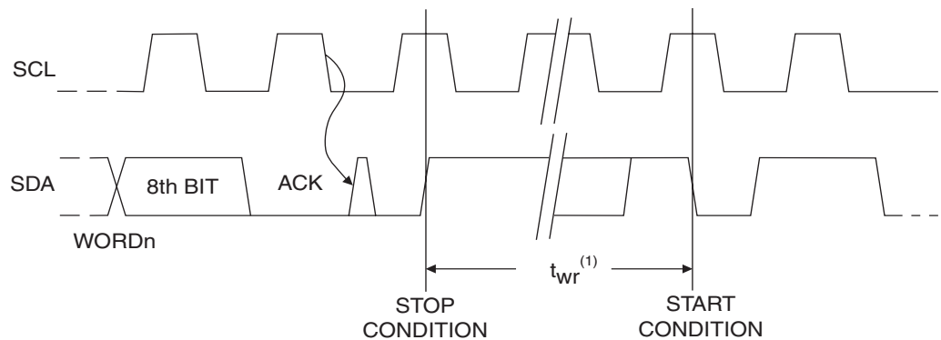
Figure 5. Write Cycle Timing
