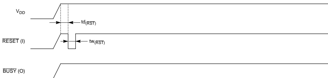
Figure 11. Power-On Timing
