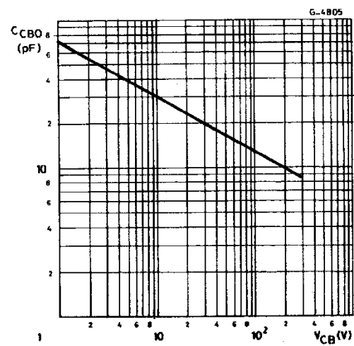
Collector-Base Capacitance
