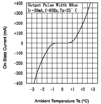
Fig.7 On-State Characteristics
