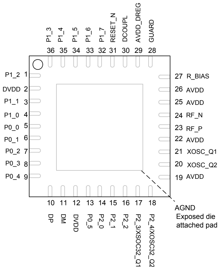
Figure 5: CC2511Fx Pinout top view
