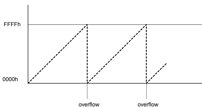
Figure 15: Free-running mode
