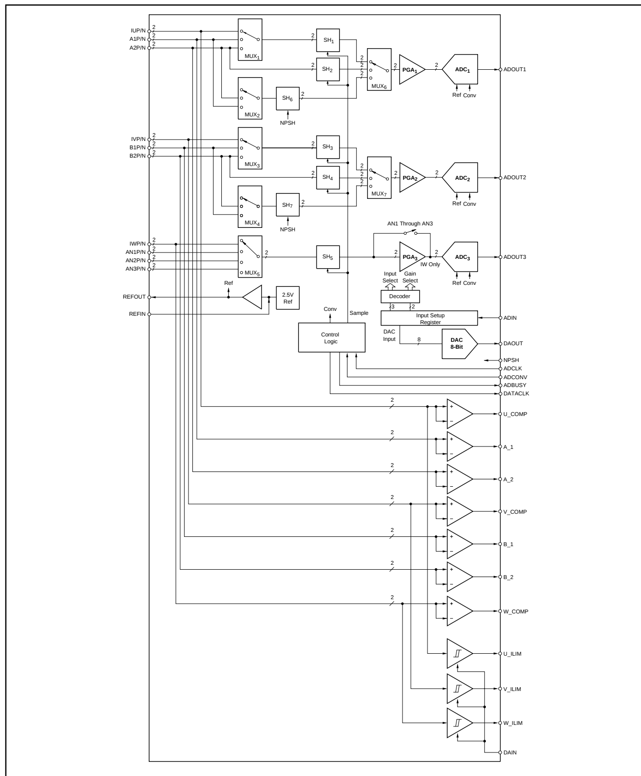
FIGURE 1. Functional Diagram.
