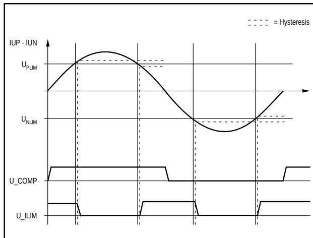
FIGURE 5. Acquisition of the Current Sign and of the Over-Current.
