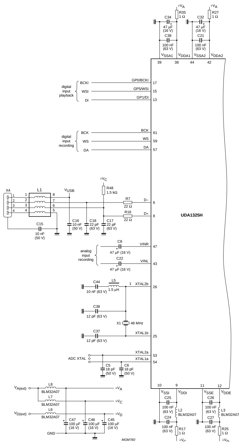
Fig.8 Application diagram UDA1325H (continued in Fig.9).
