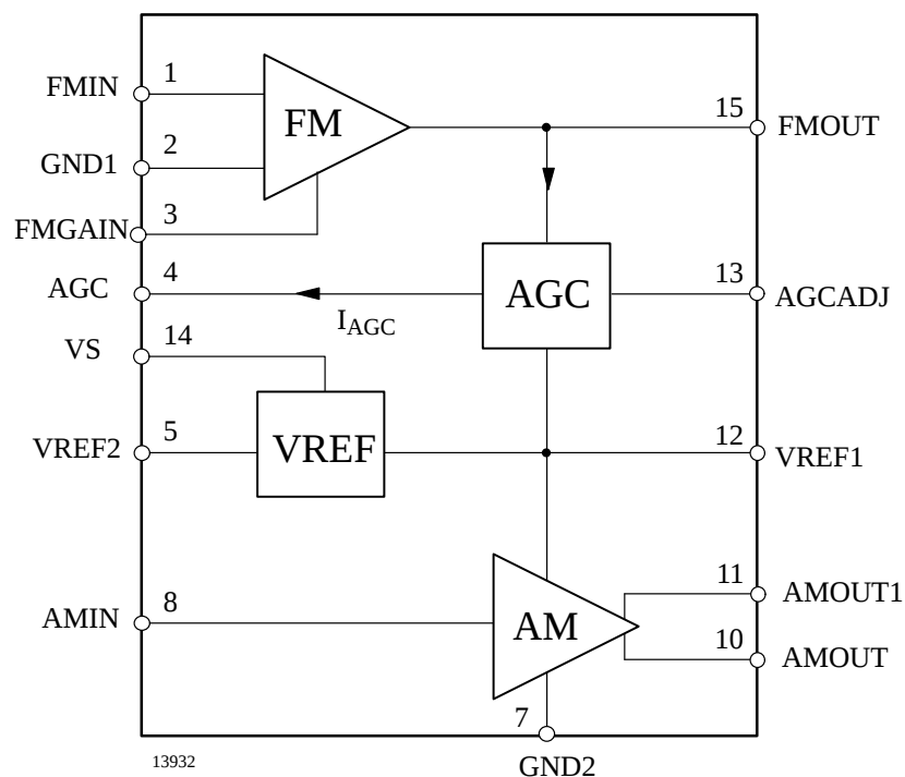
Figure 1. Block diagram
