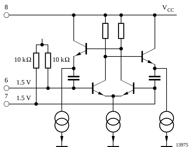
Figure 5. Pins 6/7: VCO
