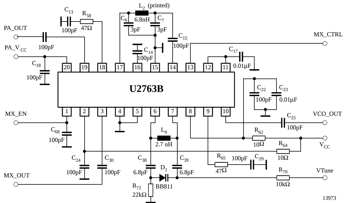
Figure 12. Application circuit
