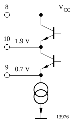
Figure 6. Pins 9/11: PLL buffer
