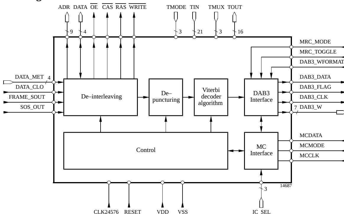
Figure 1. Block diagram
