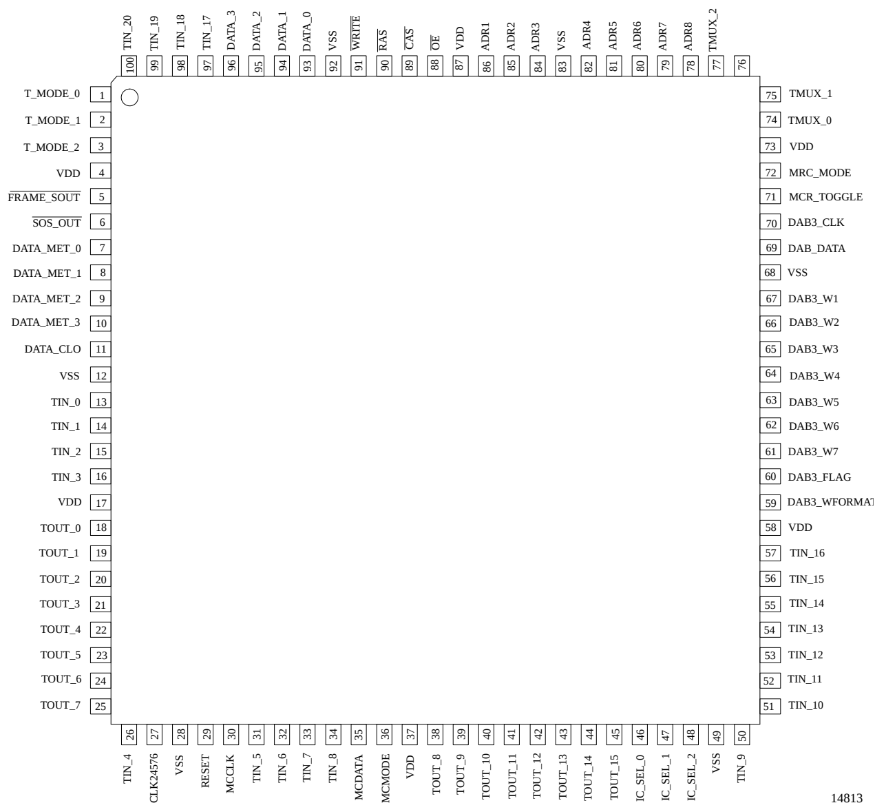
Figure 2. Pinning
