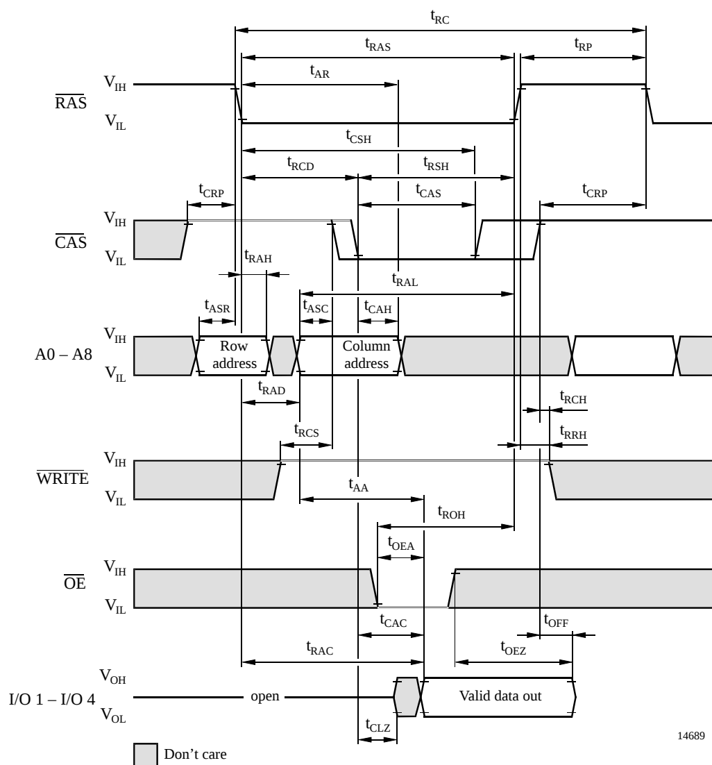
Figure 4. Read cycle
