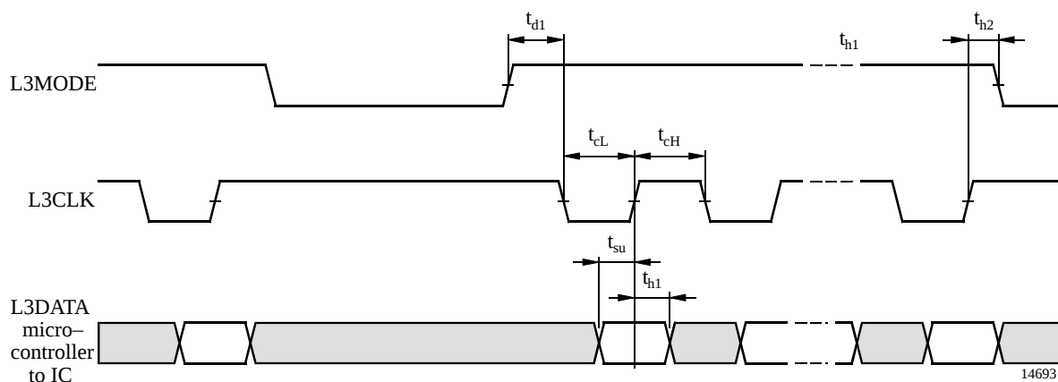
Figure 8. Timing data mode (slave receiver)
