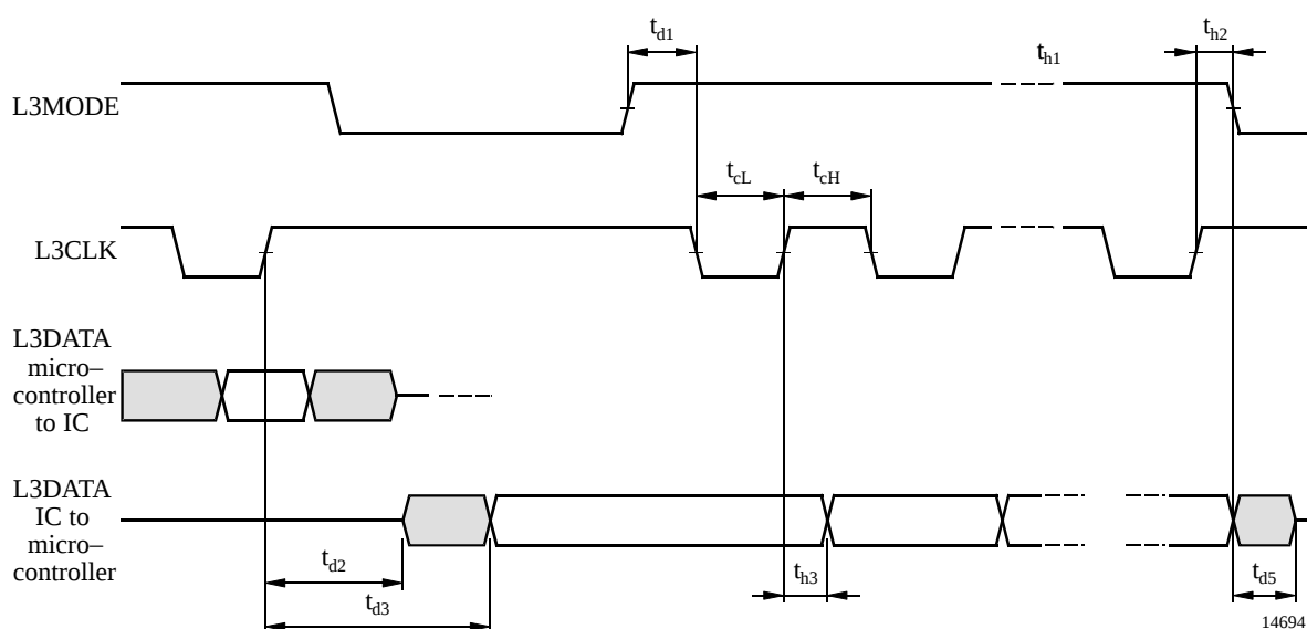
Figure 9. Timing data mode (slave transmitter)
