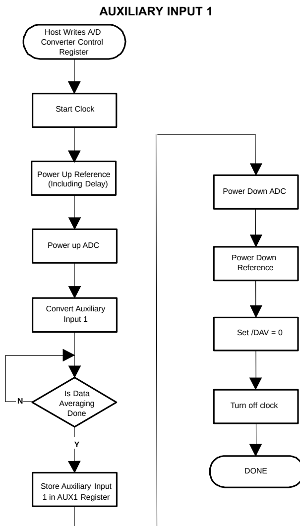
Figure 67. AUX1 Measurement Process
