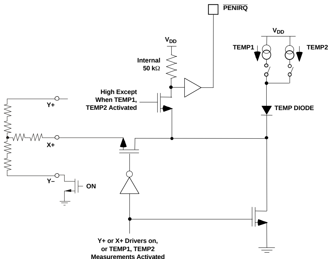
Figure 49. PENIRQ Functional Block Diagram
