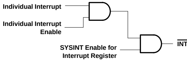
Figure 4–11. Interrupt Hierarchy
