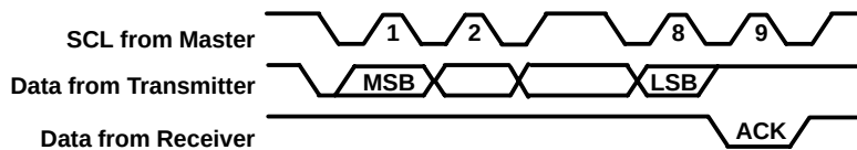
Figure 3–26. Two-Wire Serial Interface Bus Protocol
