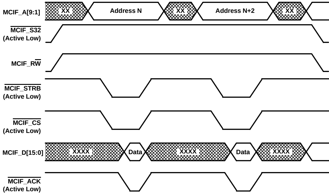
Figure 3–2. 16-Bit Read
