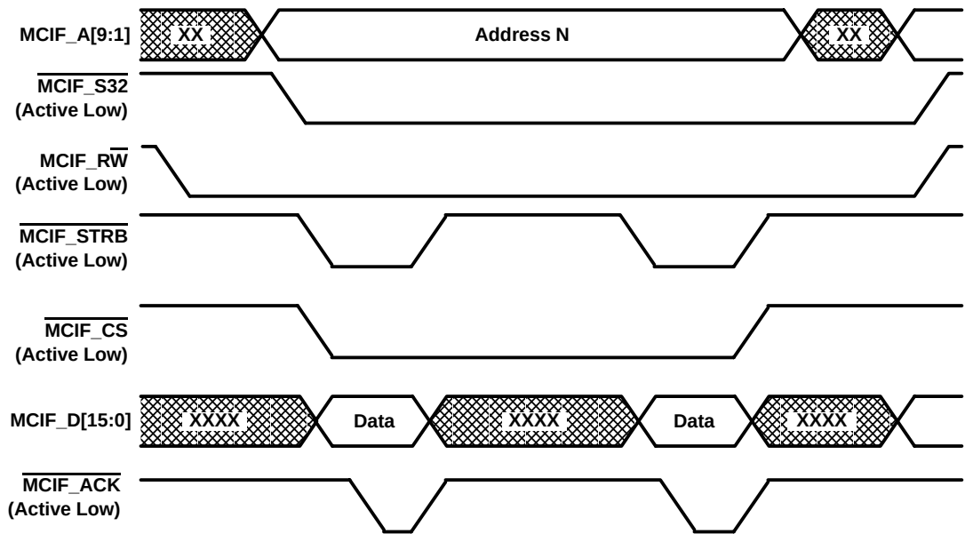
Figure 3–5. 32-Bit Write
