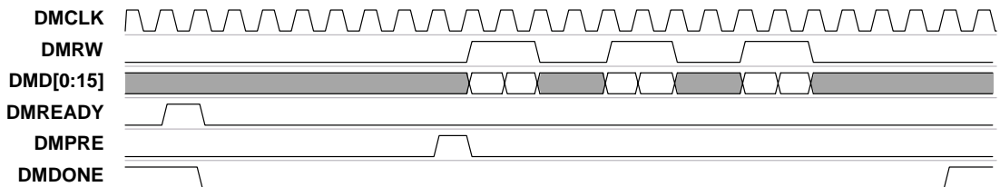
Figure 5–14. Isochronous Transmit With Auto Header Insertion at 200 Mbps
