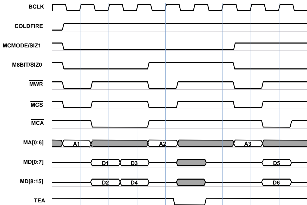
Figure 3–14. ColdFire Write
