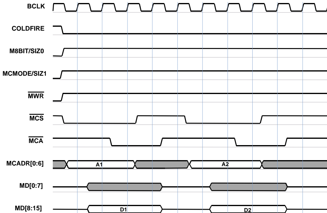
Figure 3–3. Byte Handshake Read
