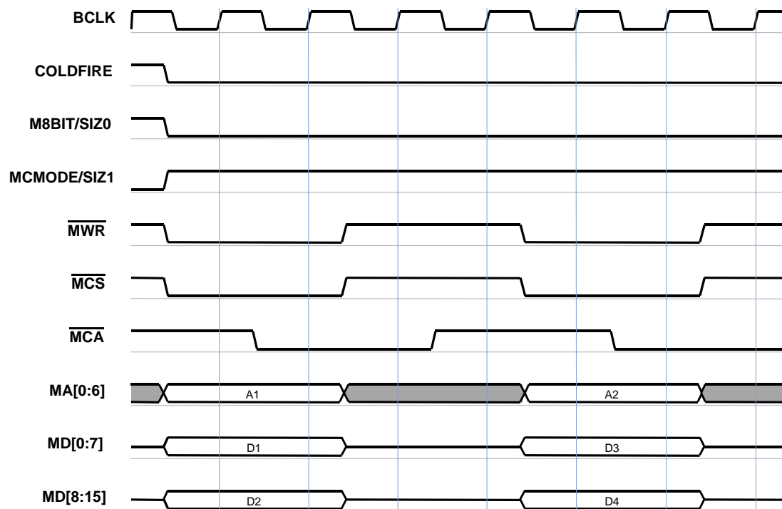
Figure 3-6. Word Handshake Write
