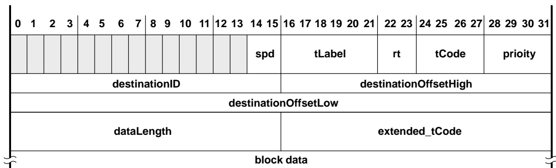
Figure 7-3. Block-Transmit Format
