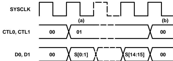
Figure 8–3. Status Transfer Timing
