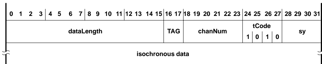
Figure 7–8. Isochronous-Transmit Format
