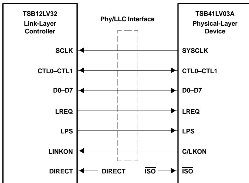
Figure 8–1. Phy-LLC Interface
