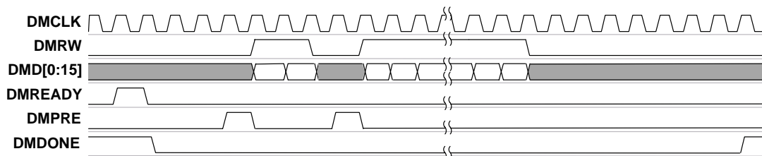
Figure 5–16. Isochronous Transmit Without Automatic Header Insertion
