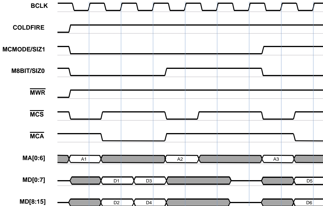
Figure 3–13. ColdFire Read
