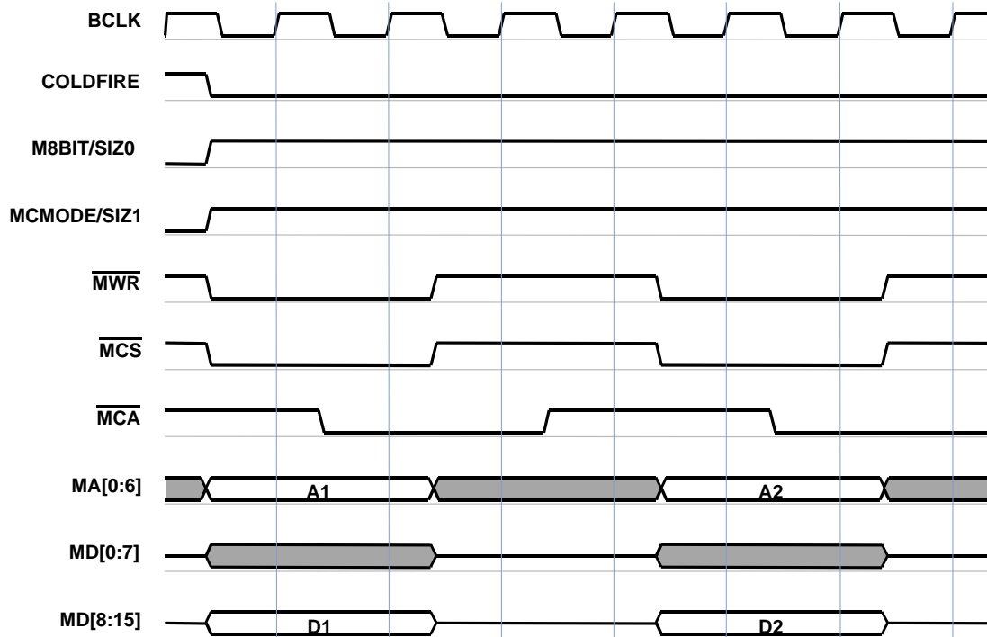
Figure 3-5. Byte Handshake Write
