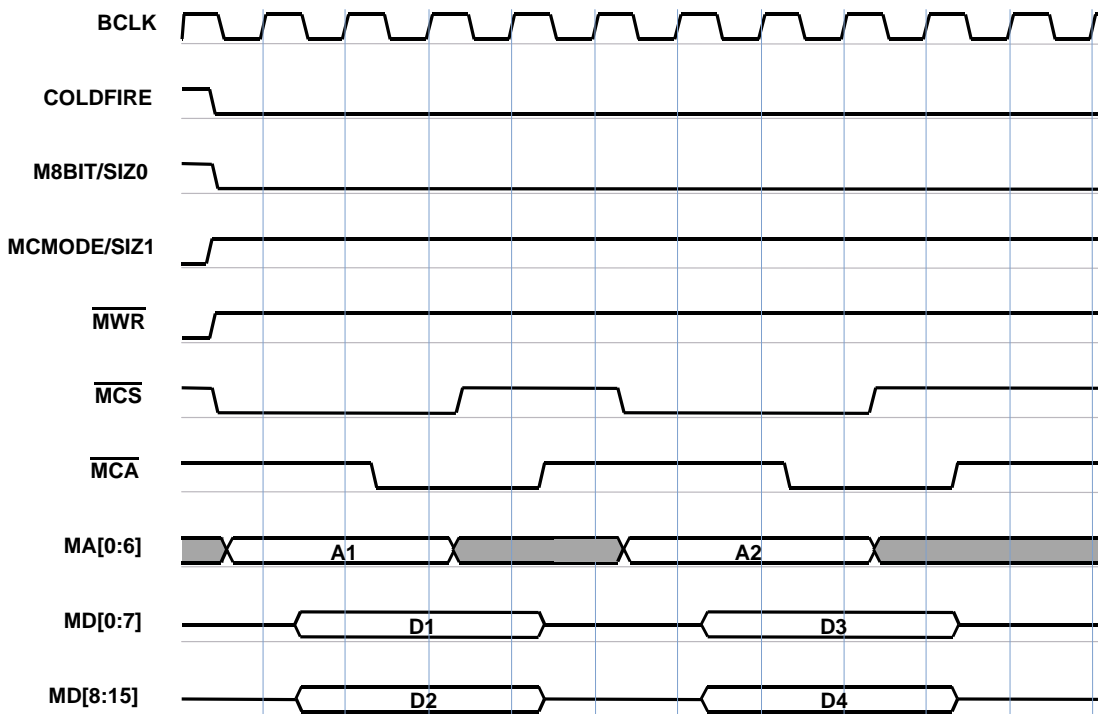
Figure 3–4. Word Handshake Read
