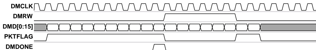
Figure 5–28. Asynchronous Block Receive Without Headers and Trailer at 400 Mbps
