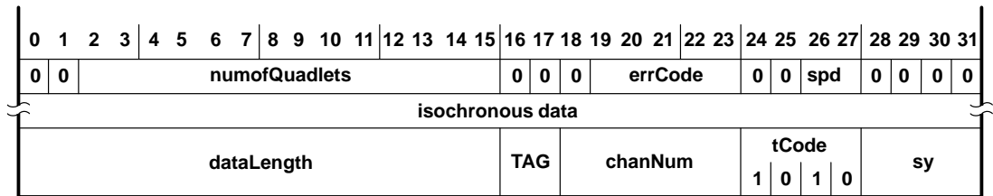
Figure 7–10. GRF Isochronous-Receive Format
