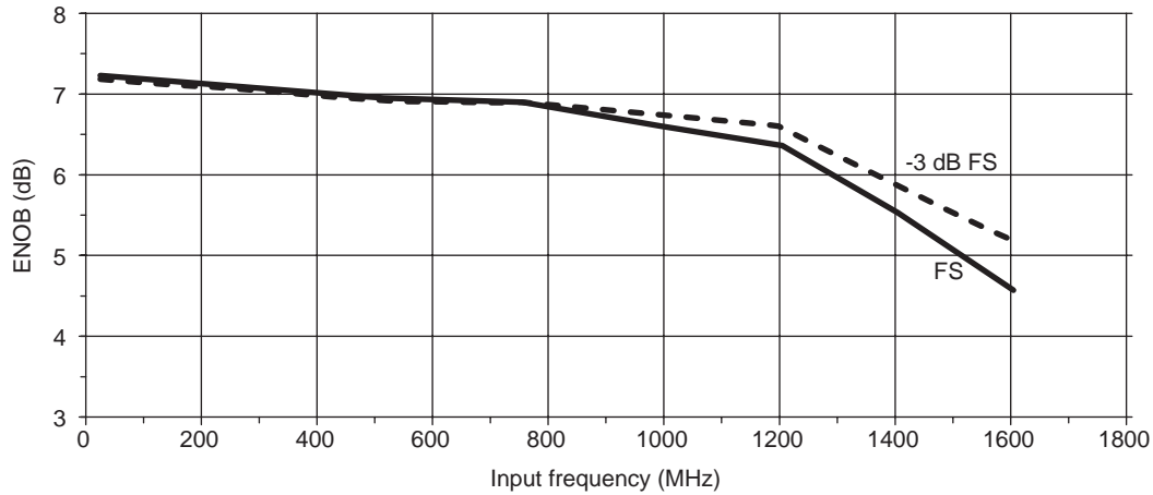
Figure 15. ENOB (dB)
