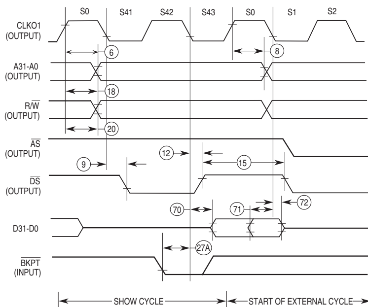
Figure 22. Background Debug Mode FREEZE Timing
