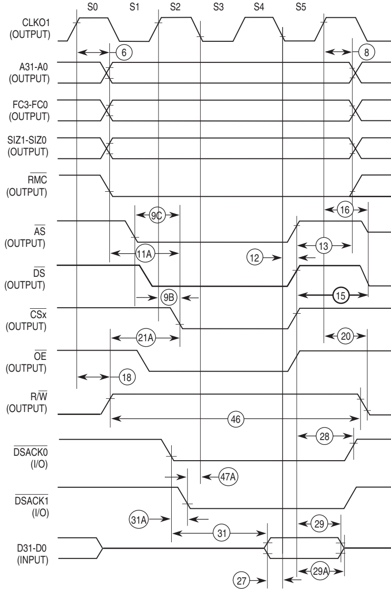
Figure 10. SRAM: Read Cycle (TRLX = 1)
