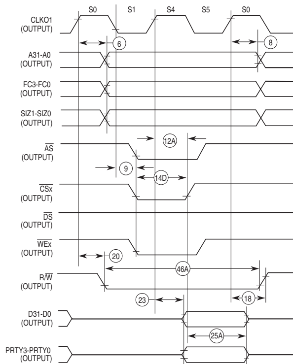
Figure 14. SRAM: Fast Termination Write Cycle (CSNTQ = 1)
