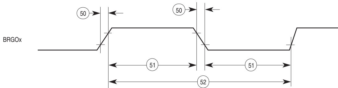
Figure 48. Baud Rate Generator Output Signals
