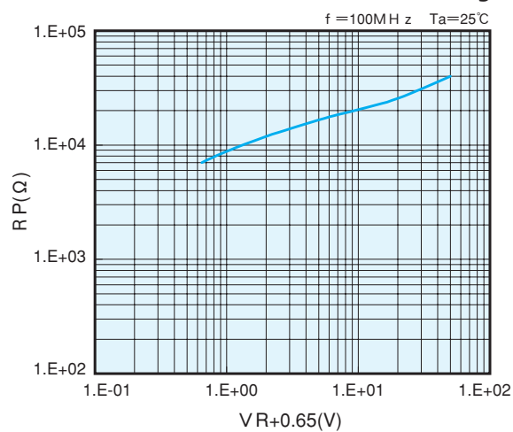
Parallel Resistance vs. Reverse Voltage
