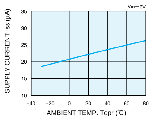
XC62GR5022 (5V HIGH SPEED)
