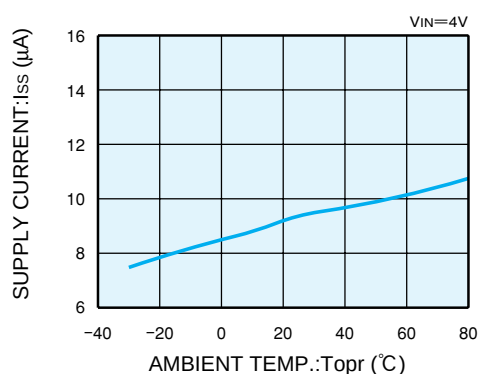
XC62GR3012 (3V)
