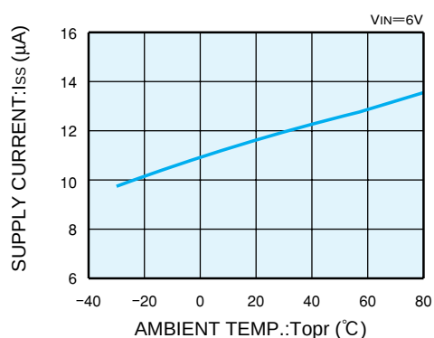
XC62GR5012 (5V)
