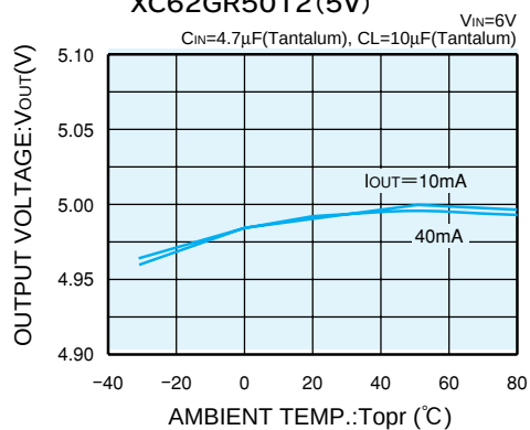
XC62GR5012 (5V)
