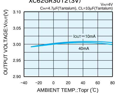
XC62GR3012 (3V)
