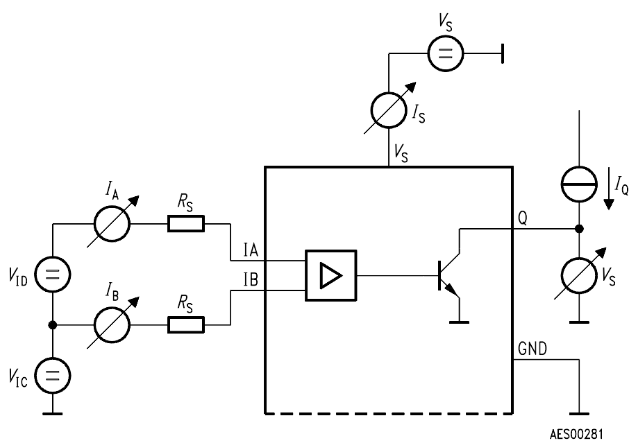
Test Circuit 2
