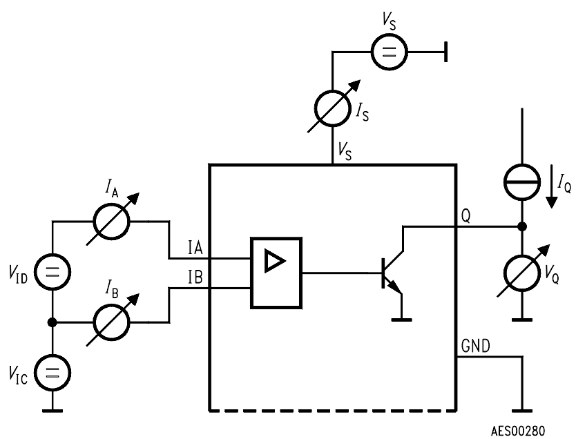
Test Circuit 1
