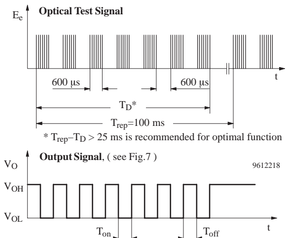
Figure 5. Output Function
