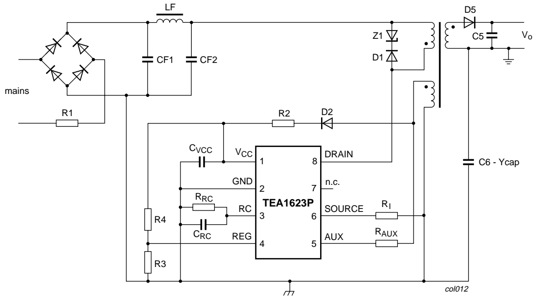
Fig 6. Application with primary sensing for TEA1623P.
