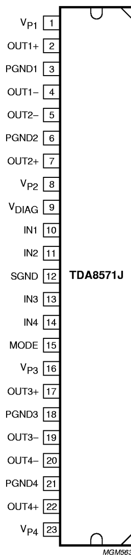
Fig.2 Pin configuration.
