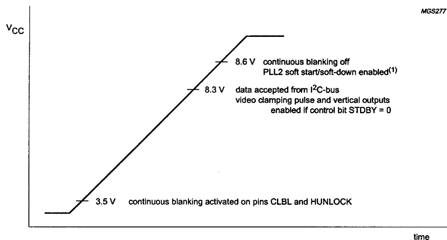
a. Start-up sequence.
