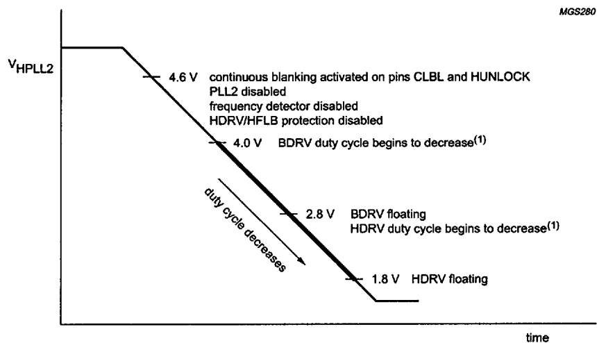
b. PLL2 soft-down sequence, if V_{CC} > 8.6 V.
