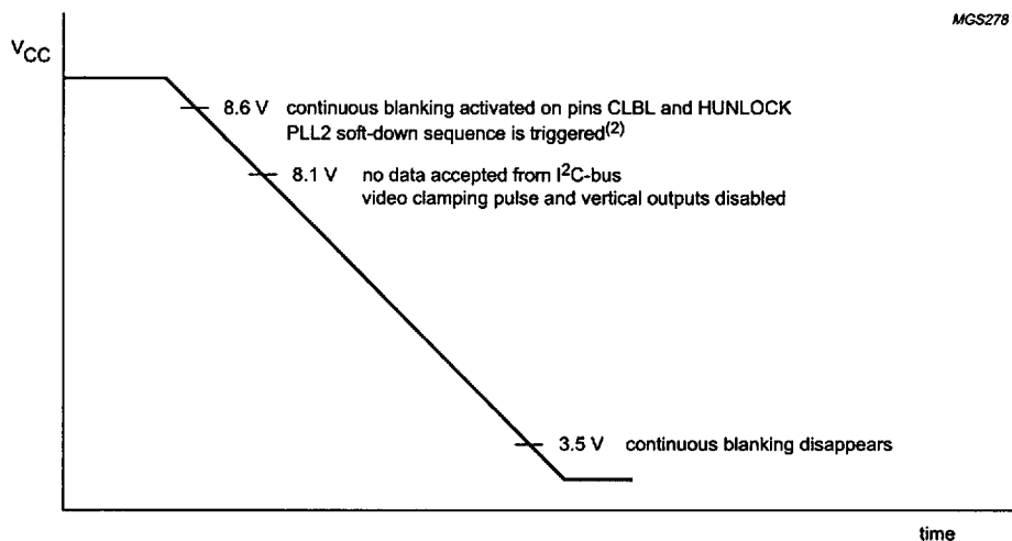
b. Shut-down sequence.
