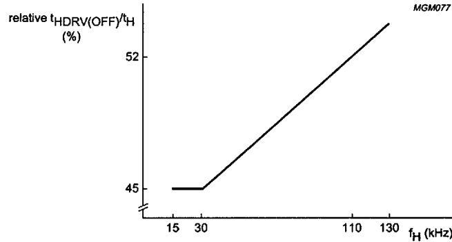
Fig. 16 Relative t_{OFF} time of HDRV versus H-frequency.
