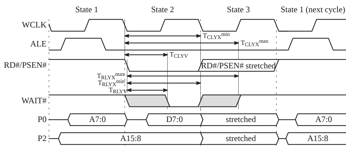
Figure 21. Real-time Synchronous Wait State: Code Fetch/Data Read
