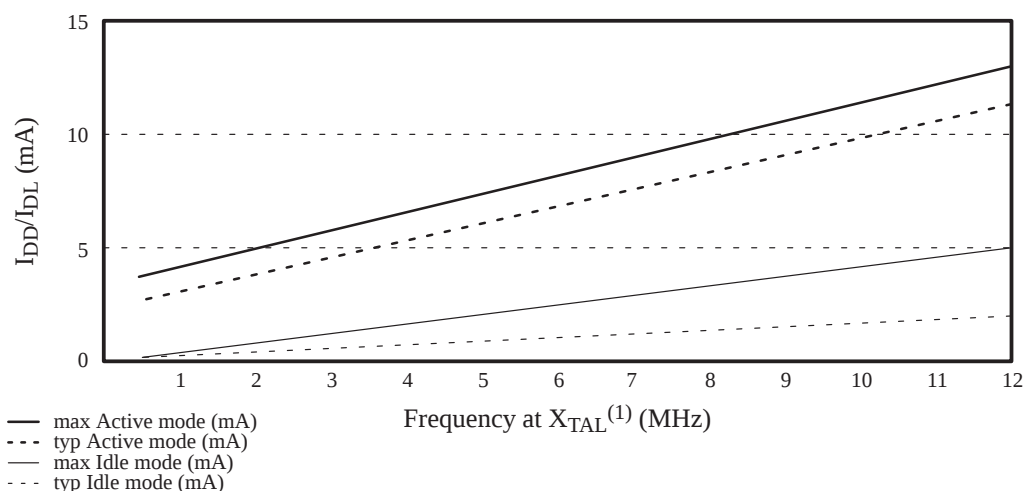
Figure 11. I_{DD}/I_{DL} versus X_{TAL} Frequency; V_{DD} = 2.7 to 5.5 V
