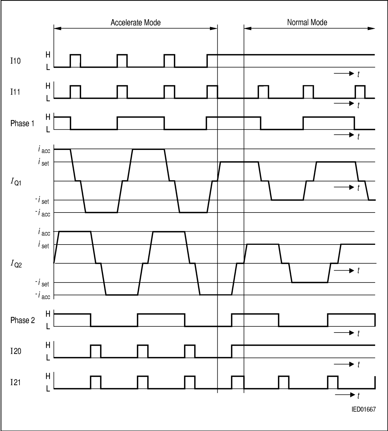
Figure 7 Half-Step Operation
