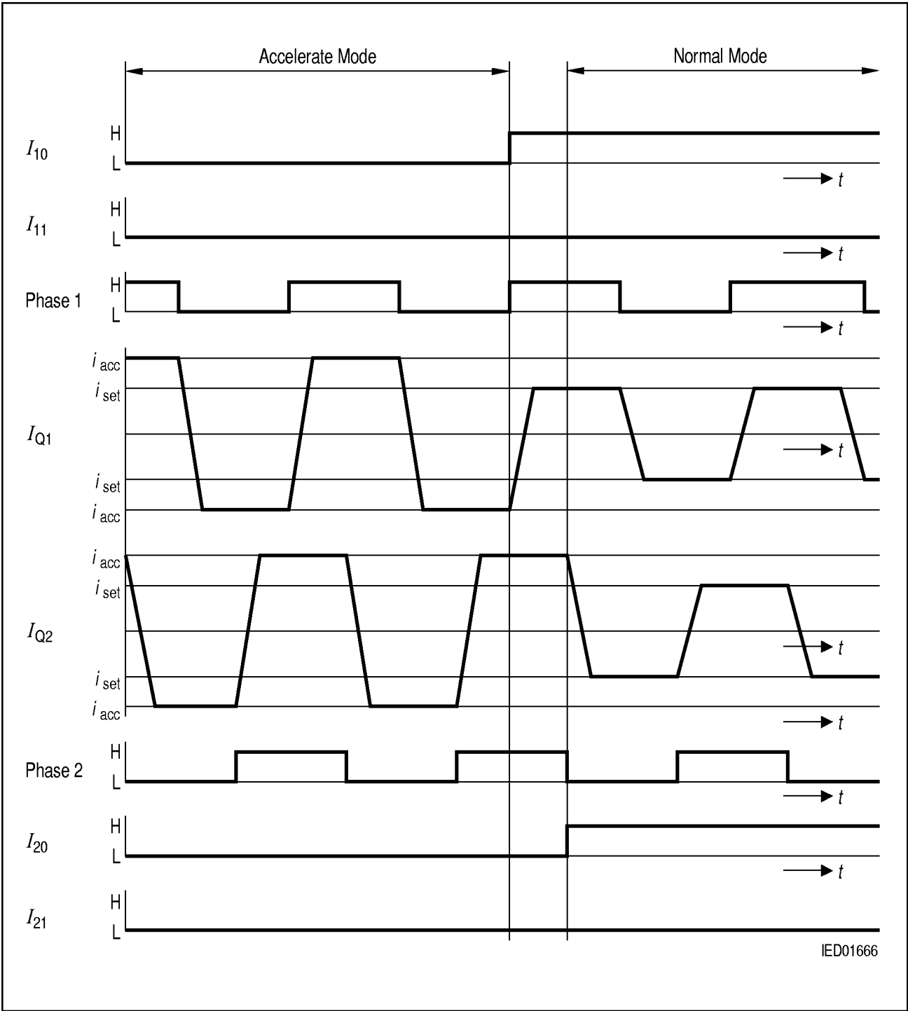
Figure 6 Full-Step Operation
