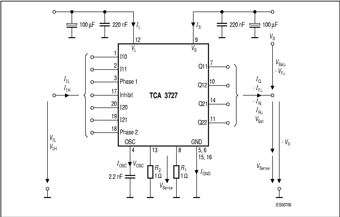
Figure 4 Test Circuit
