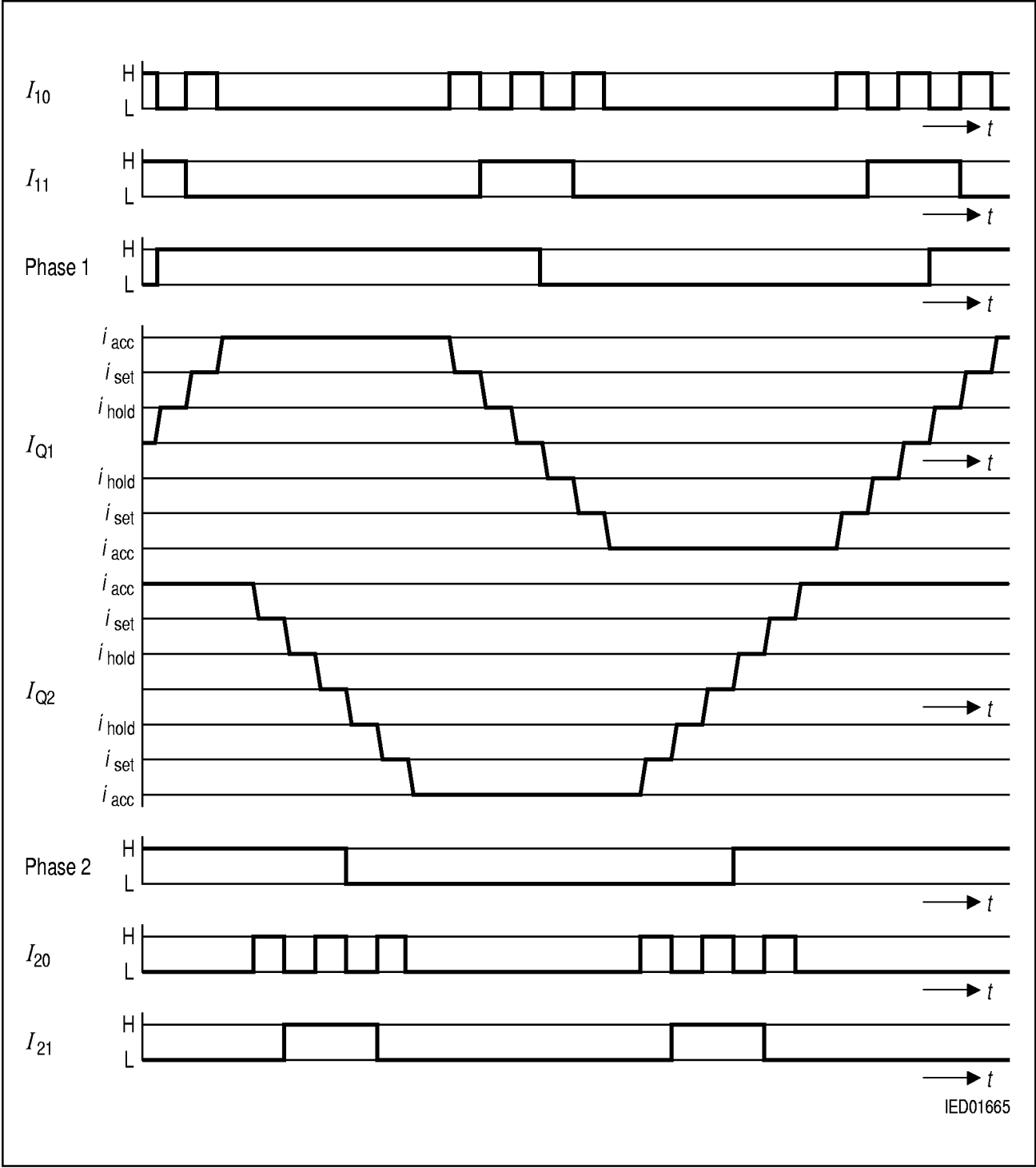
Figure 9 Mini-Step Operation
