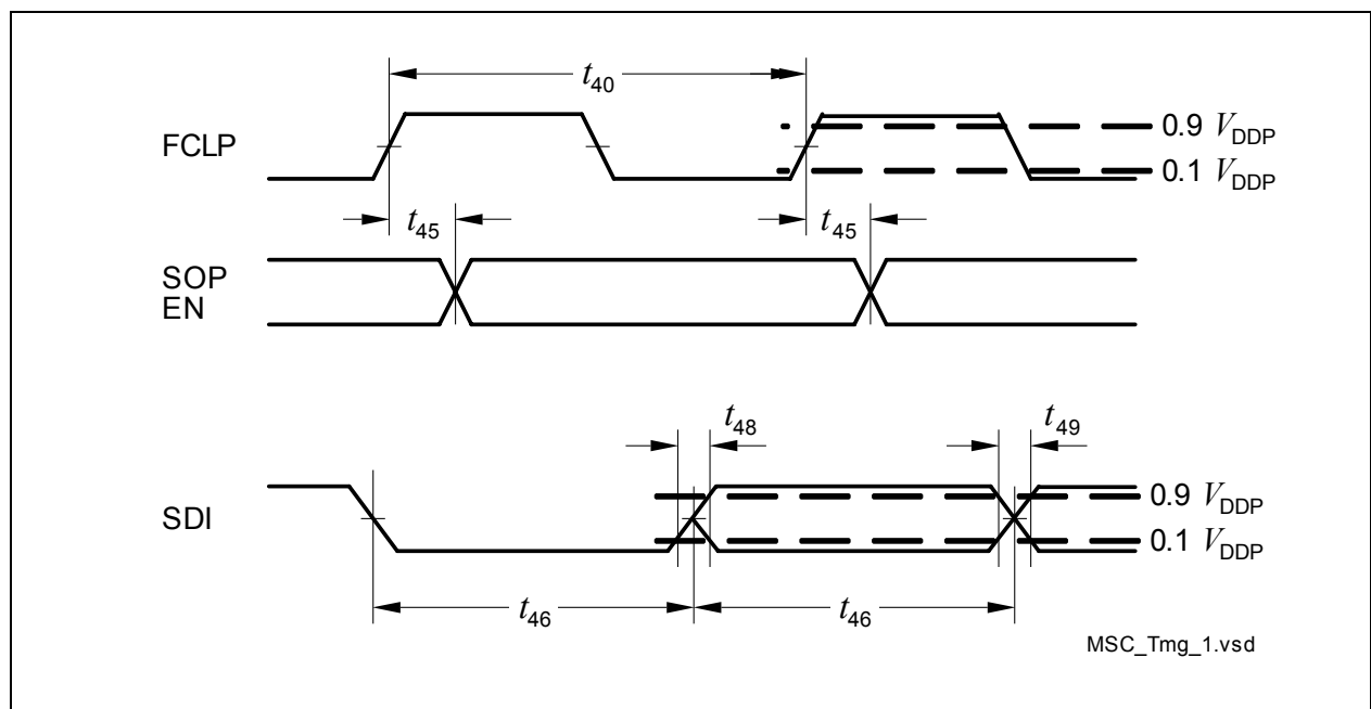
Figure 4-14 MSC Interface Timing
