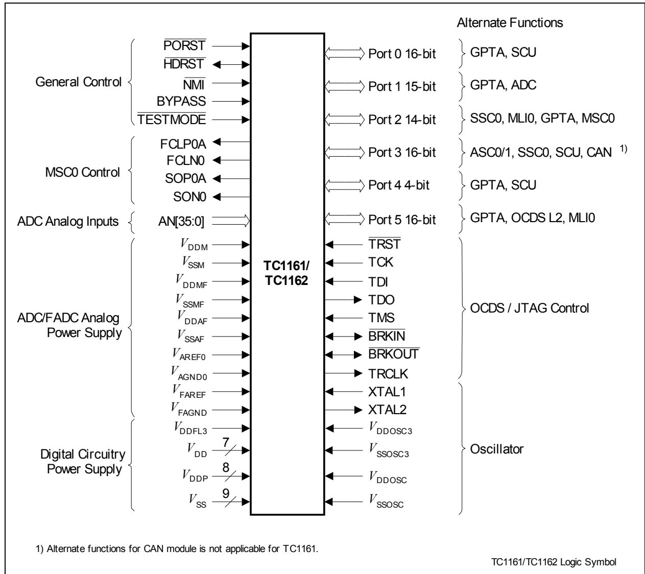
Figure 2-2 TC1161/TC1162 Logic Symbol
