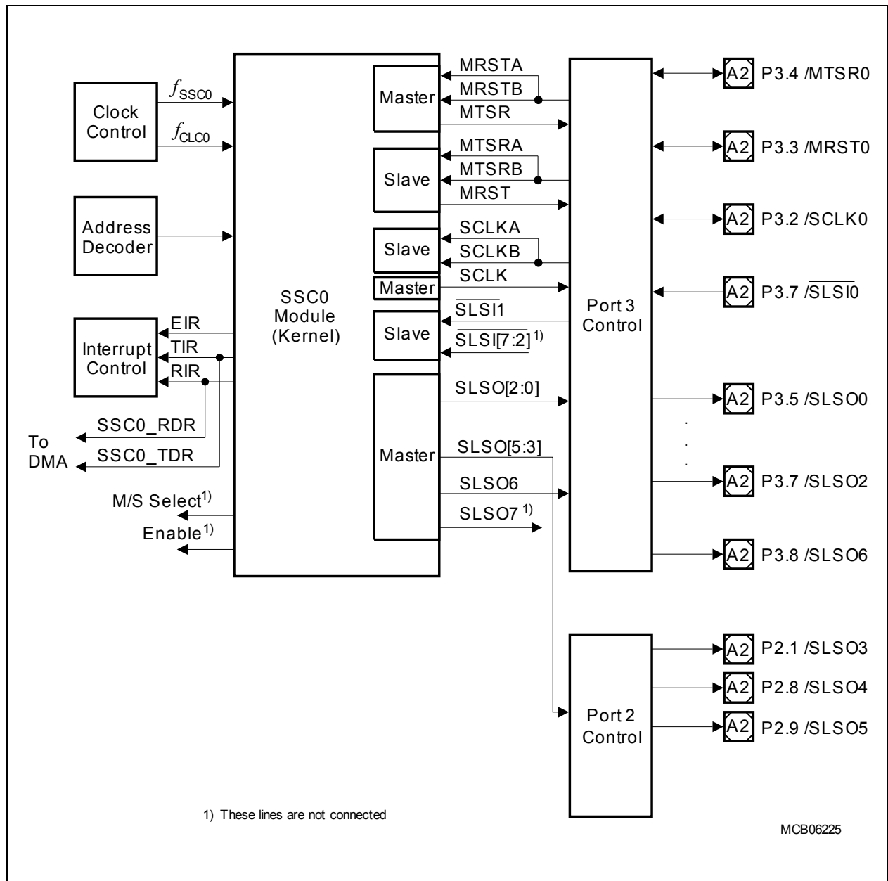
Figure 3-4 Block Diagram of the SSC Interfaces
