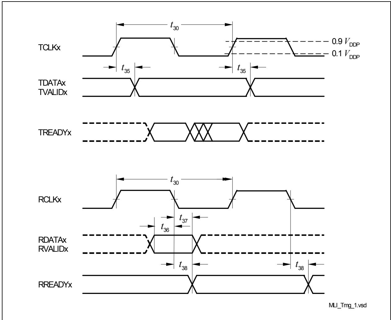
Figure 4-13 MLI Interface Timing
