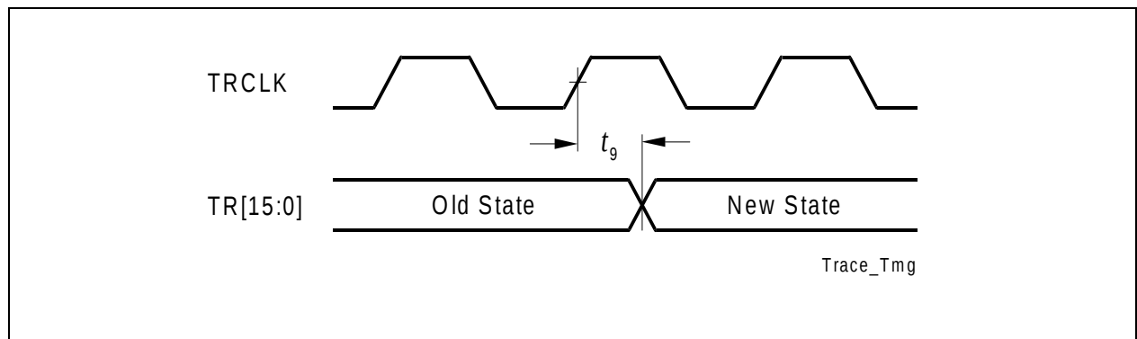
Figure 4-12 Debug Trace Timing
