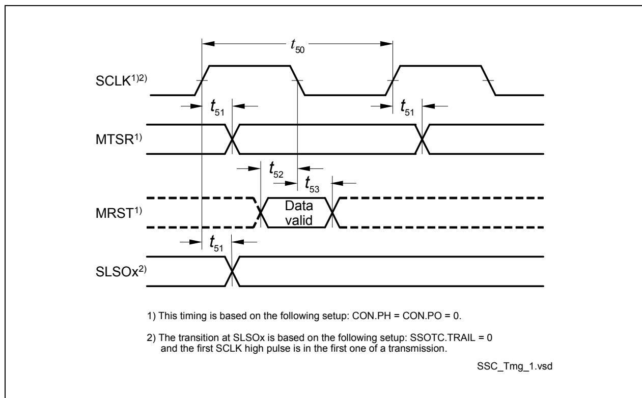
Figure 4-15 SSC Master Mode Timing
