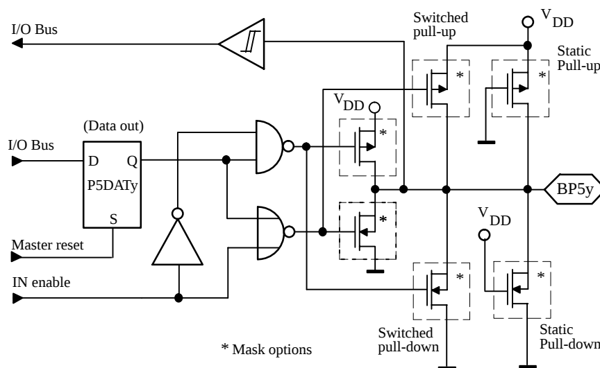
Figure 24. Bidirectional Port 5
