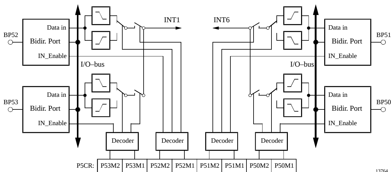
Figure 25. Port 5 external interrupts
