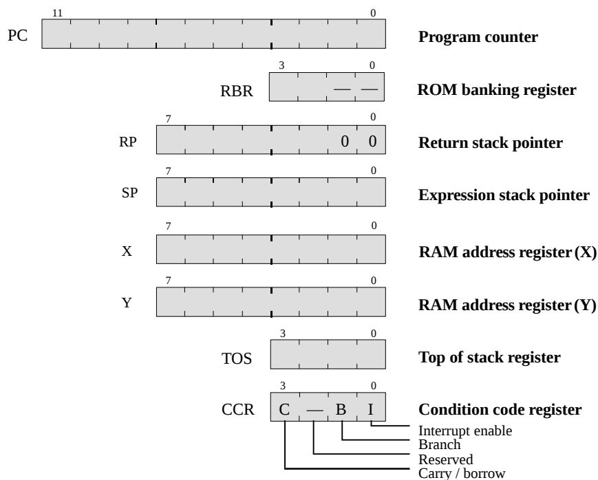
Figure 6. Programming model
