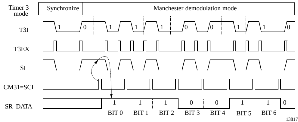
Figure 53. Manchester demodulation
