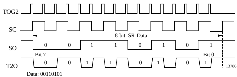
Figure 40. Biphase modulation
