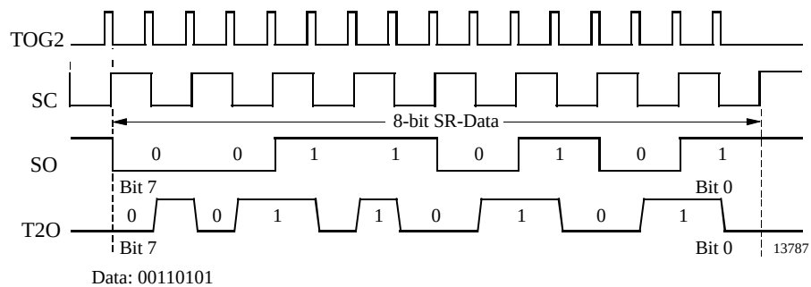
Figure 41. Manchester modulation
