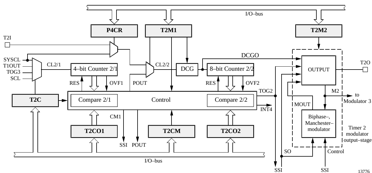
Figure 30. Timer 2
