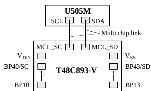
Figure 66. Multi-chip link
