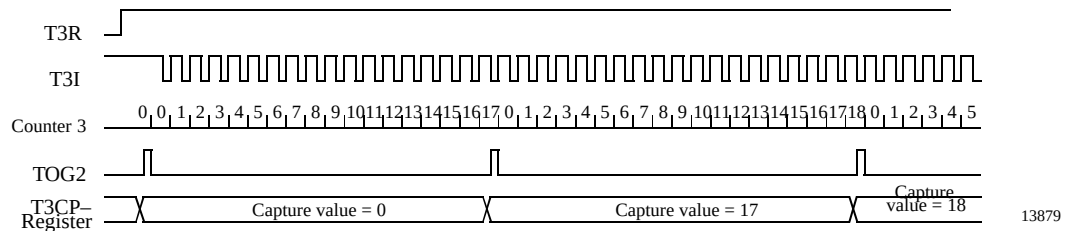
Figure 80. Frequency measurements
