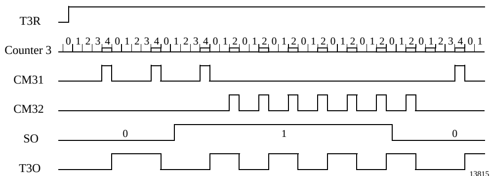
Figure 51. FSK modulation
