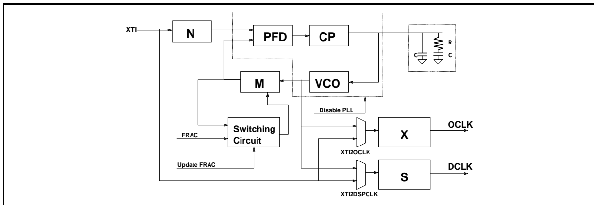
Figure 6. PLL and Clocks Generation System
