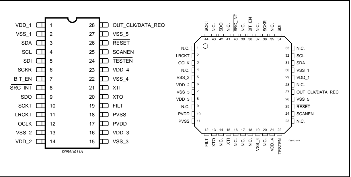
Figure 2. PIN CONNECTION
