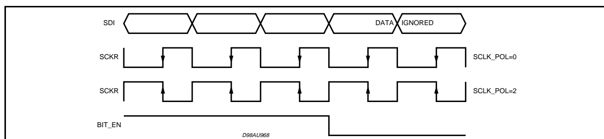
Figure 5. Serial Input Interface Clocks
