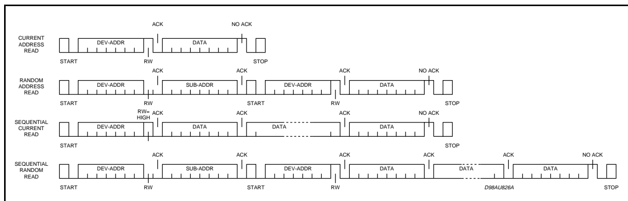
Figure 10. Read Mode Sequence
