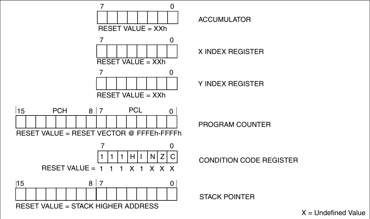
Figure 11. CPU Registers
