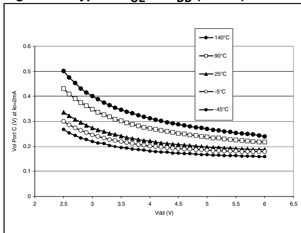
Figure 94. Typical V_{OL} vs V_{DD} (Port C)
