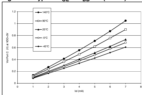
Figure 88. Typical V_{OL} at V_{DD}=5V (Port C)
