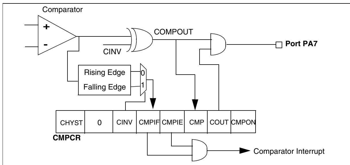
Figure 62. Analog Comparator
