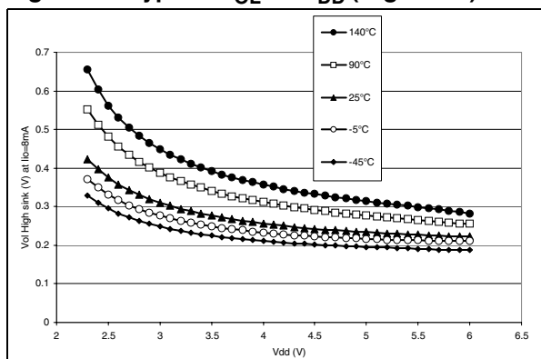
Figure 93. Typical V_{OL} vs V_{DD} (High-sink)
