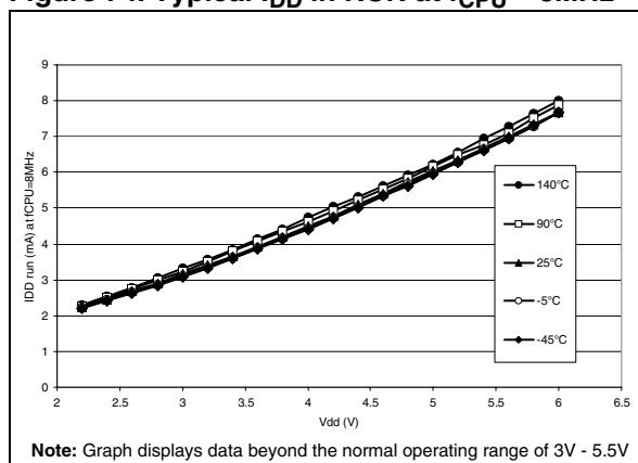
Figure 74. Typical I_{DD} in RUN at f_{CPU} = 8\text{MHz}
