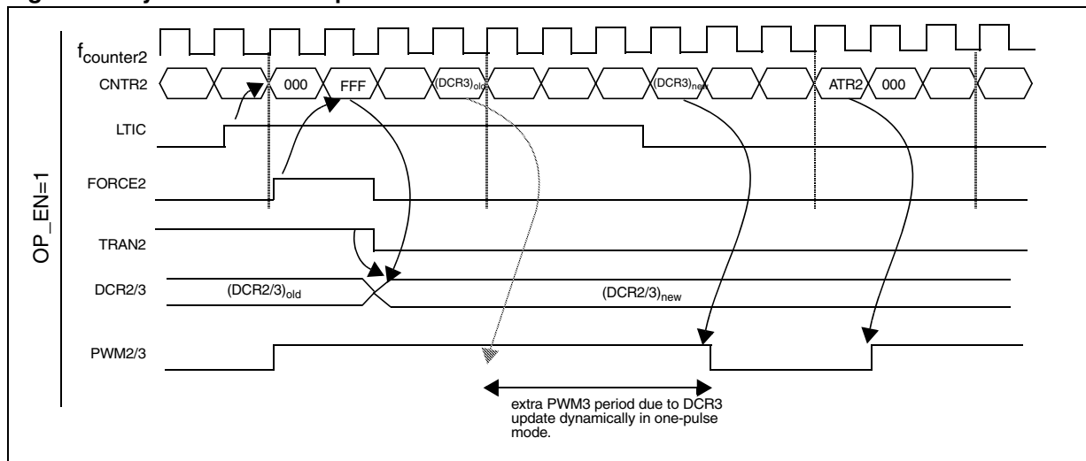
Figure 49. Dynamic DCR2/3 update in One Pulse Mode
