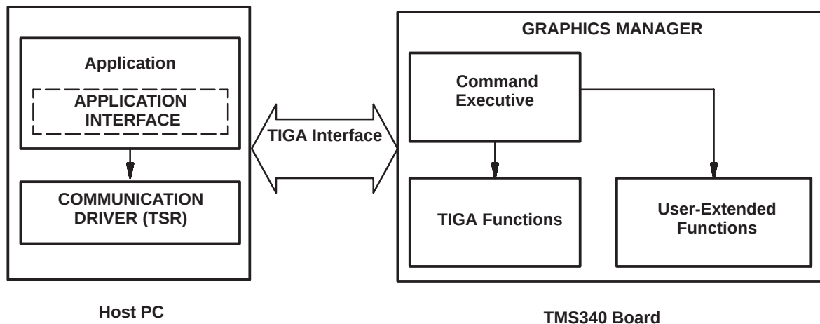
Figure 1–1. Block Diagram
