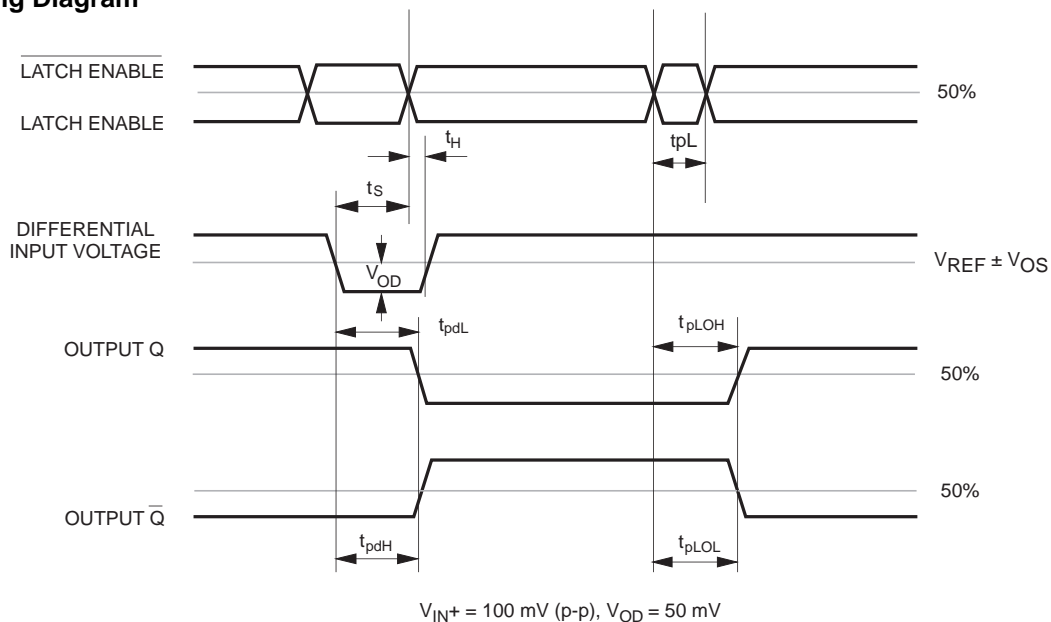
Figure 1 - Timing Diagram
