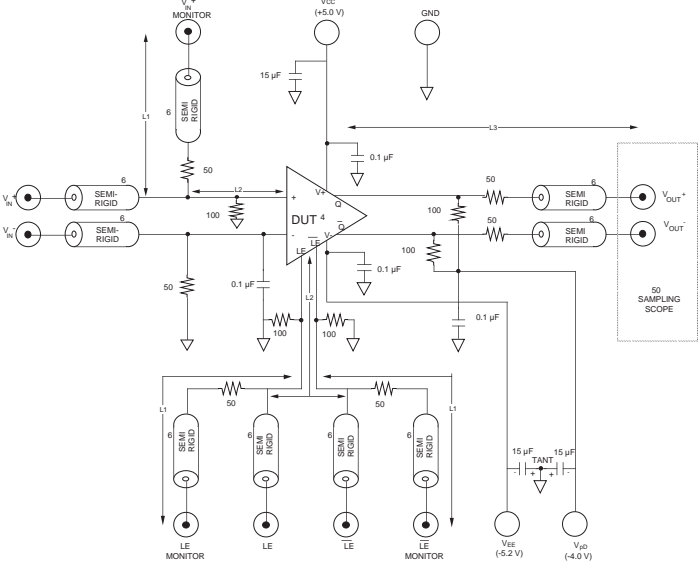
Figure 8 - Test Load
