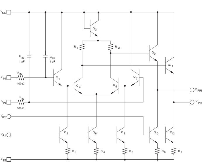
Figure 7 - Output Circuit
