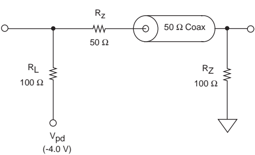
Figure 8 - Test Load
