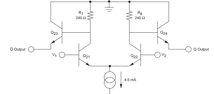
Figure 7 - Output Circuit
