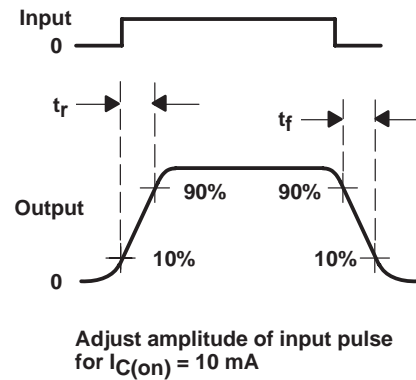
VOLTAGE WAVEFORMS
