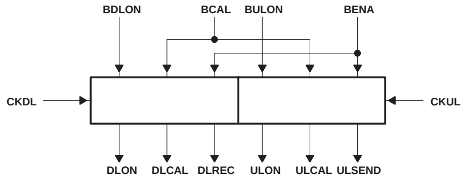
Figure 4–12. Timing Interface
