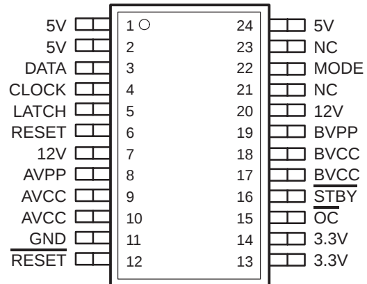
DB PACKAGE (TOP VIEW)
