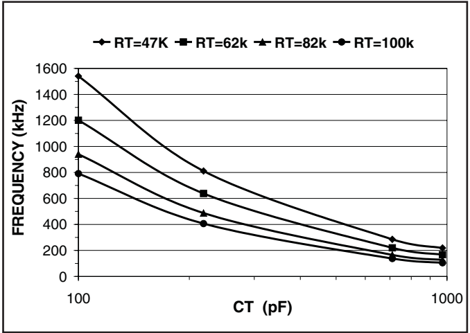
Figure 8. Frequency vs. RT/CT (oscillator frequency).
