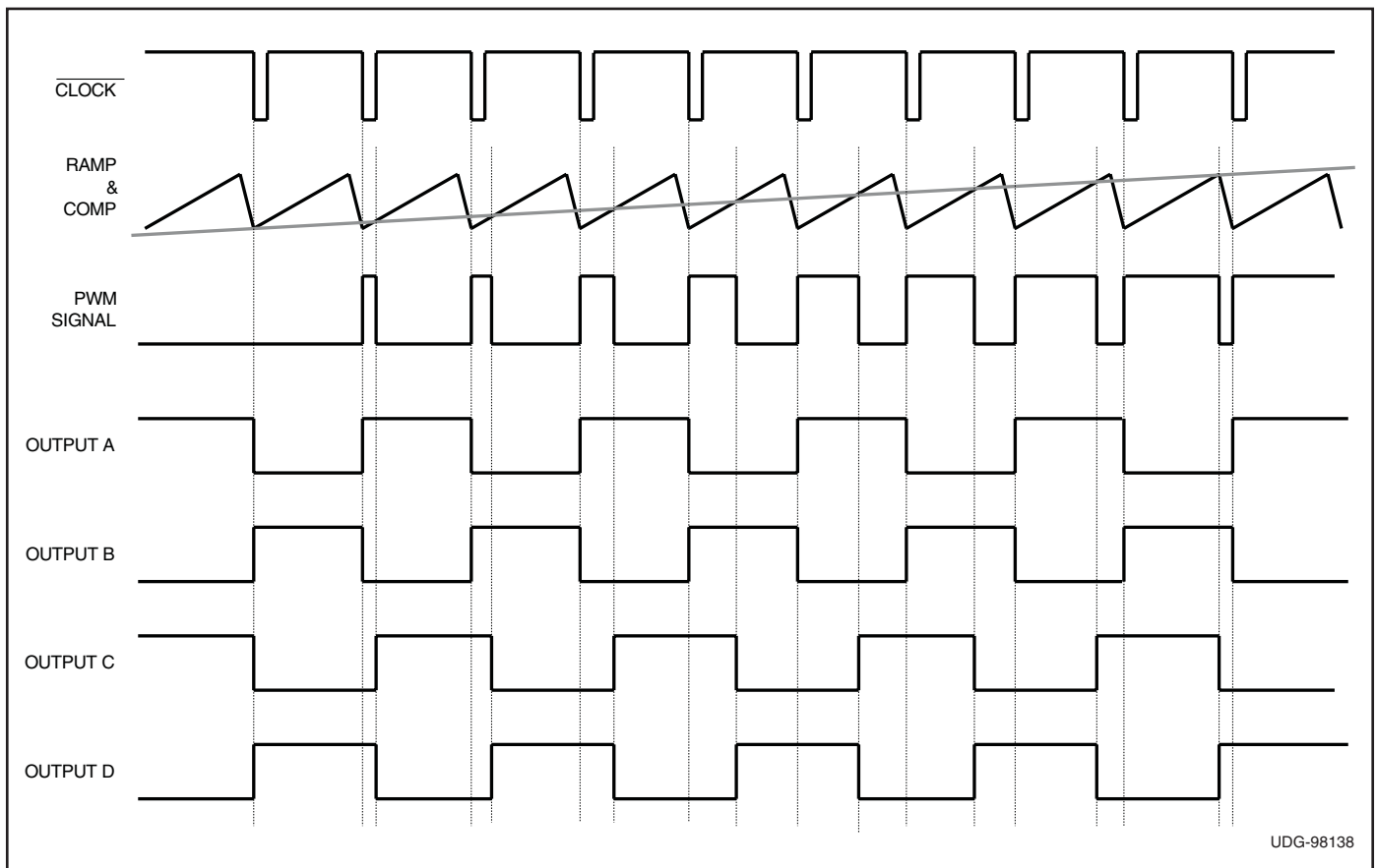
Figure 4. UCC3895 timing diagram (no output delay shown).
