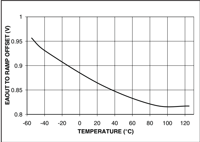
Figure 6. EAOUT to RAMP offset over temperature.
