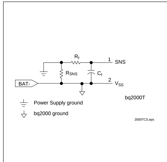
Figure 9. Current-Sensing Circuit
