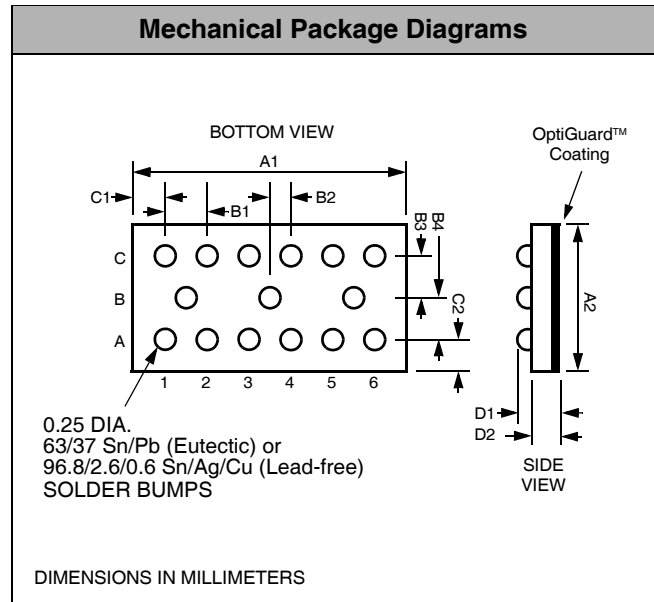
Package Dimensions for CM1441 Chip Scale Package
