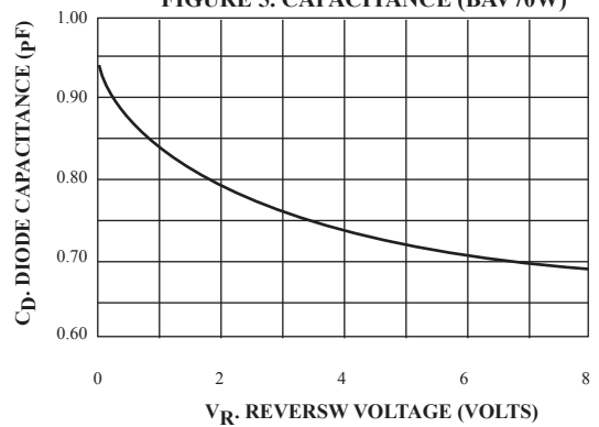
FIGURE 5. CAPACITANCE (BAV70W)
