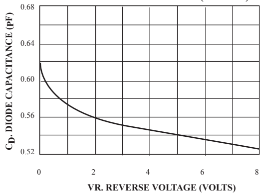
FIGURE 4. CAPACITANCE(BAS16W)
