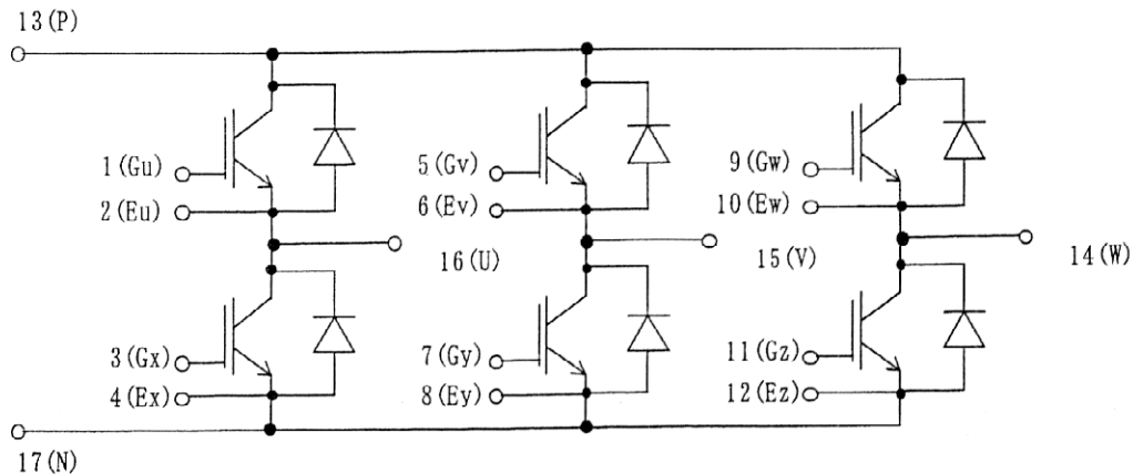
2. Equivalent circuit
