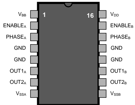
16 Lead Plastic DIP
