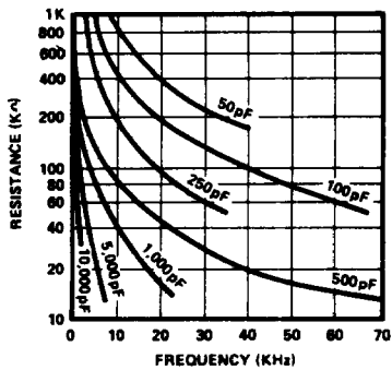
RESISTANCE vs OSCILLATOR FREQUENCY
