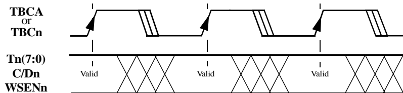
Figure 3: Transmit Timing, TMODE(2:0) = 10X
