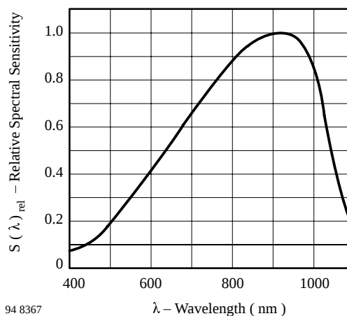
Figure 10. Relative Spectral Sensitivity vs. Wavelength
