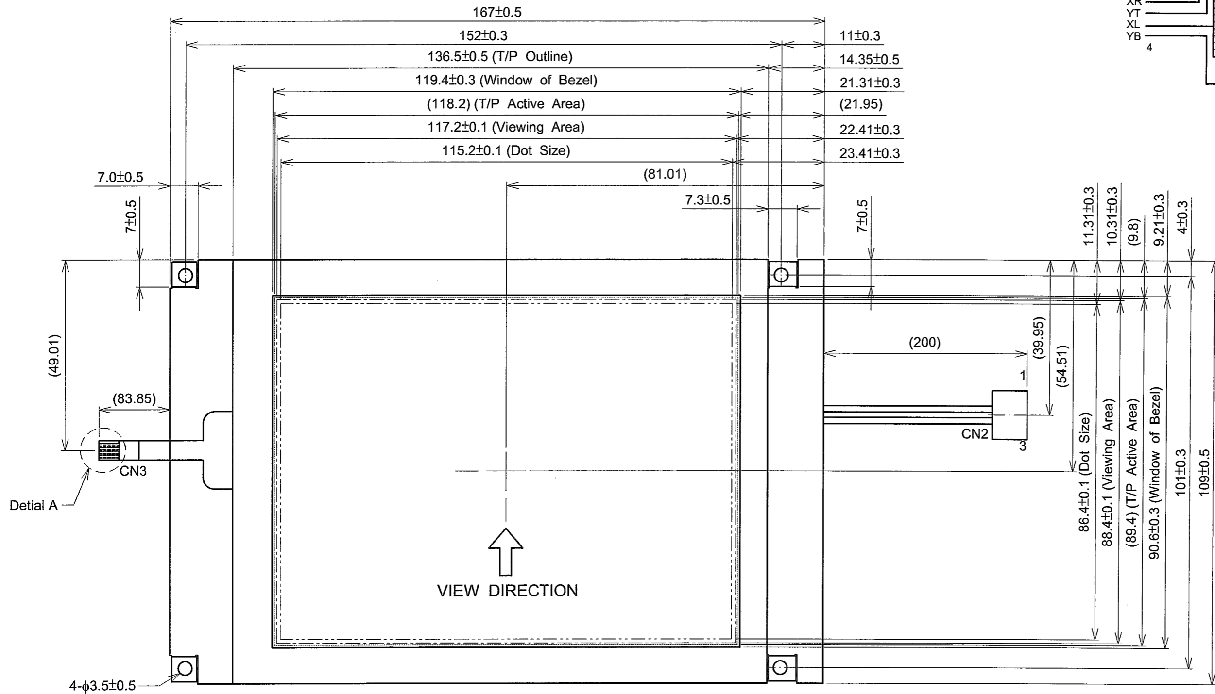
Top View
