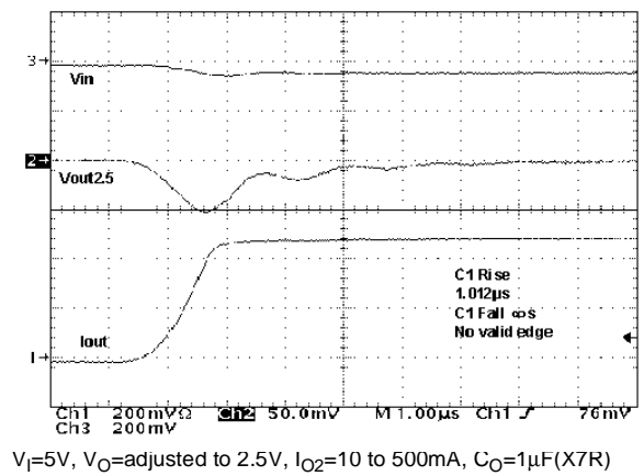
Figure 23 : Load Transient
