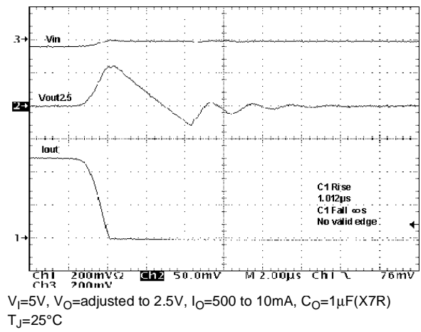
Figure 23 : Load Transient
