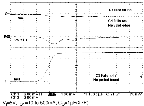
Figure 24 : Load Transient
