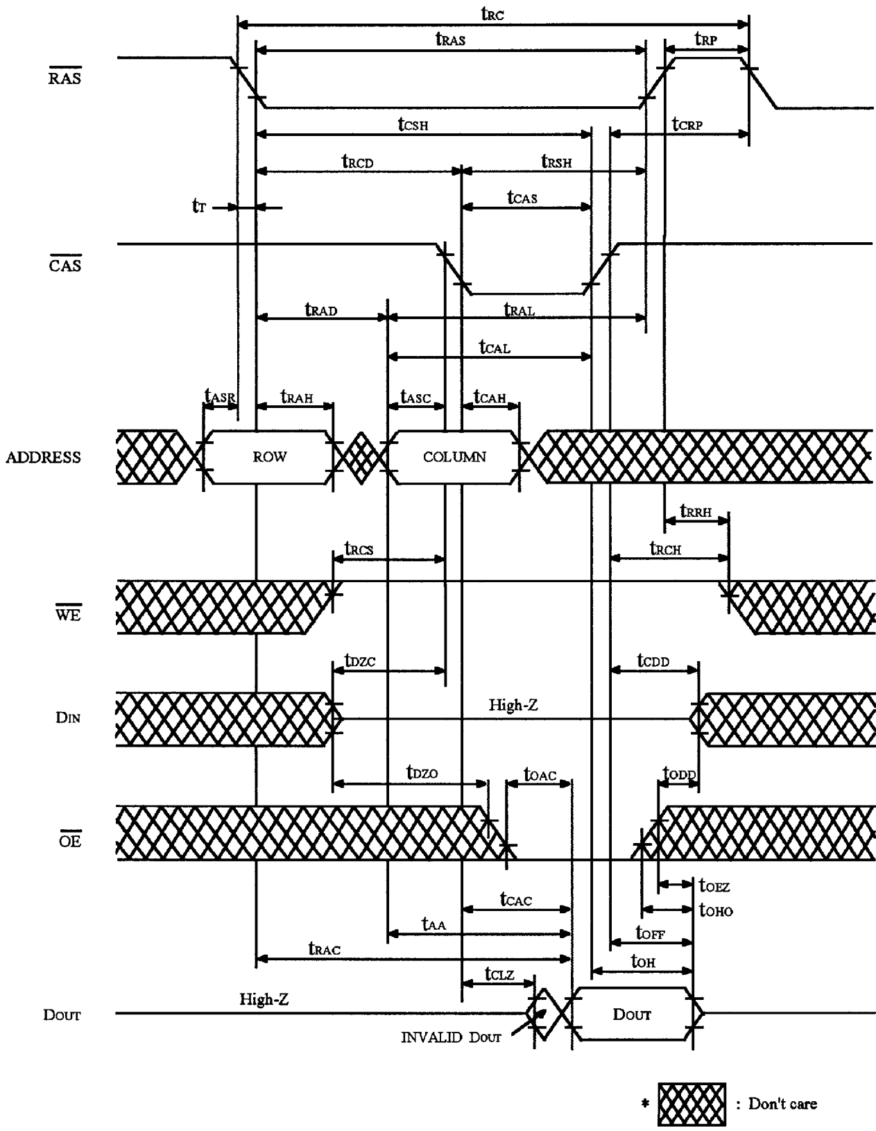
FIGURE 1. READ CYCLE
